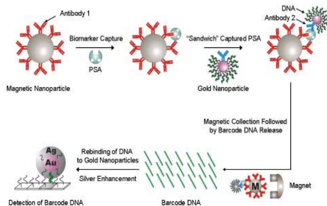
Figure III-2. The biobarcode assay uses two particle probes that are each specific to the targeted biomarker. One is a magnetic particle probe that captures the target from complex media. The other is a gold nanoparticle probe that is specific to the target of interest but that also carries with it hundreds to thousands of DNA sequence barcodes chosen to be specific to the target of interest. Released biobarcode DNA can be detected using common DNA detection methods (microarray, fluorescence, electrochemistry). (Image credit: Chad Mirkin, Northwestern University.)
