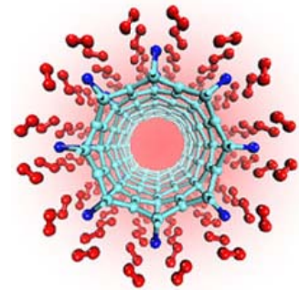
Figure III-4. This computer model shows how titanium atoms (dark blue) can attach above the centers of single-walled carbon nanotubes (light blue). Each titanium atom can bond with four hydrogen molecules (red), which could lead to efficient fuel cells for future automobiles. (Image credit: T. Yildirim, NIST, and S. Ciraci, Bilkent University, Turkey.)
