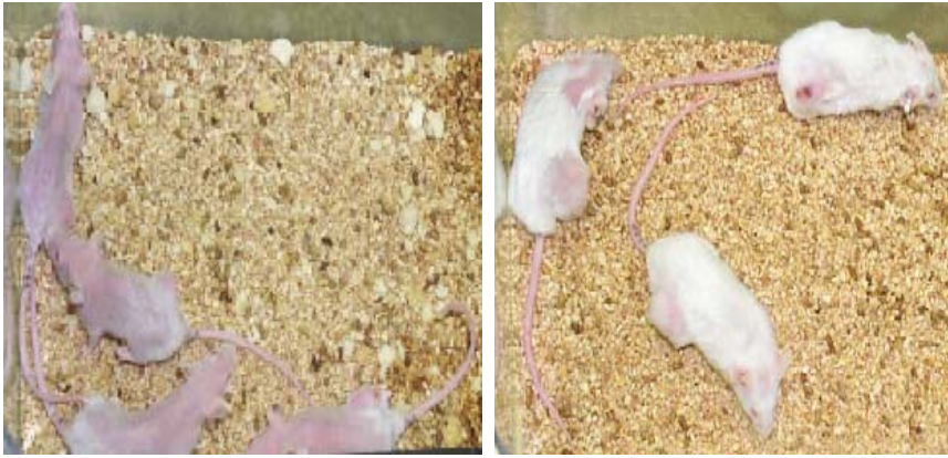
Figure III-3. (Left image) Mice receiving free methotrexate (30 mg/kg) alone lost their hair, lost weight, and experienced other toxic side effects from the drug. (Right image) Mice given nanoparticle-delivered methotrexate to shrink their tumors did not lose their hair—a common side effect of anticancer drugs. (Image credit: Kukowska-Latello, Michigan Nanotechnology Institute for Medicine and Biological Sciences.)
